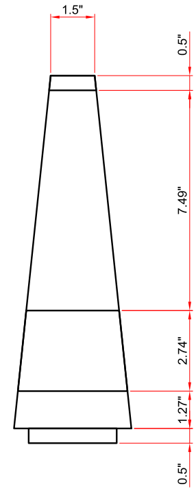
REAR
