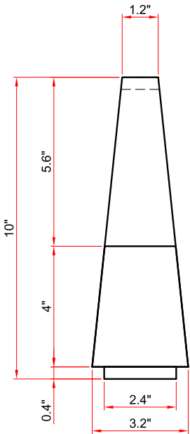
FRONT
