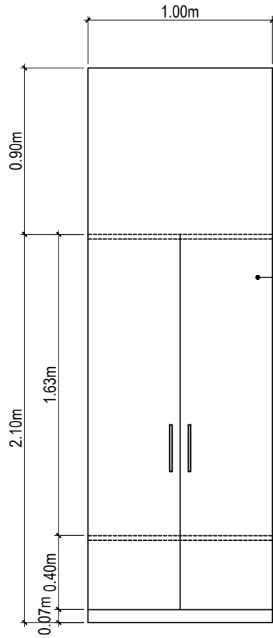
2 - CLOAK CABINET 1 UNIT
