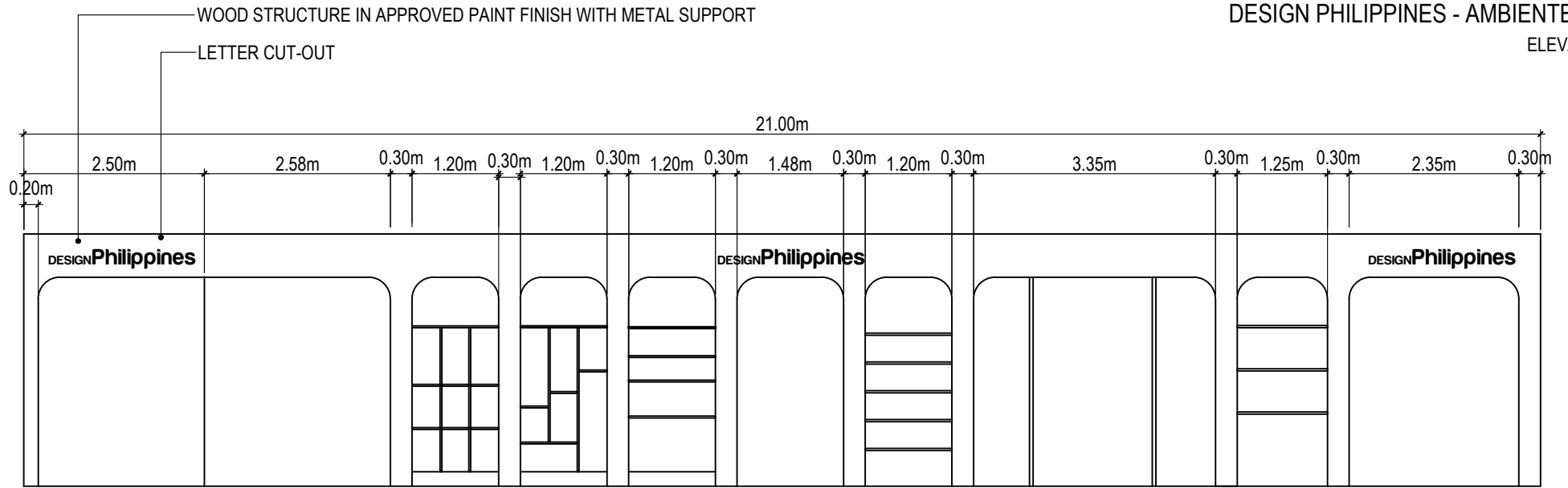
ELEVATION C
