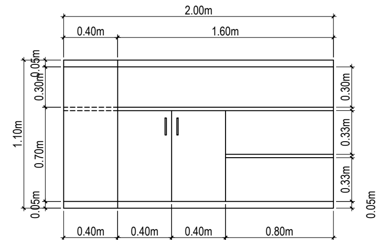
REAR VIEW
